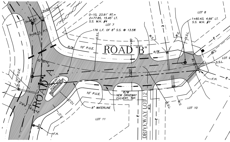
PRELIMINARY-PLAN-ROAD "B"
