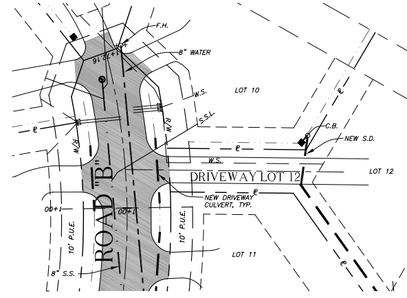
PRELIMINARY-PLAN-DRIVEWAY LOT 12
