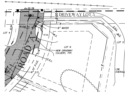
PRELIMINARY-PLAN-DRIVEWAY LOT 5
